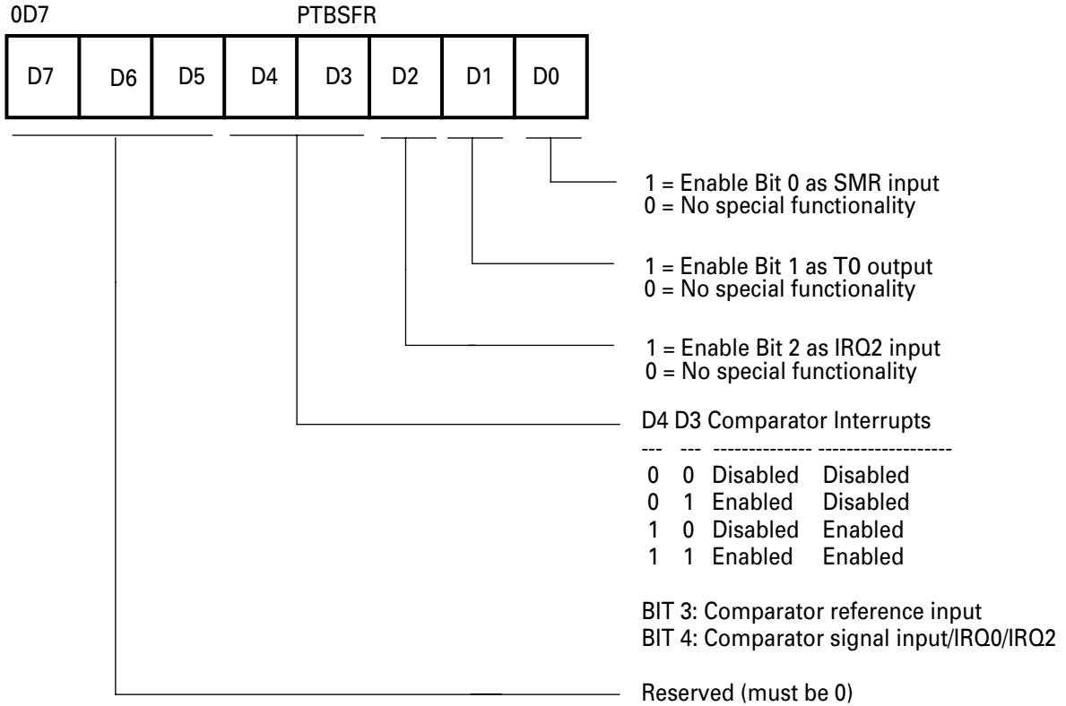
Figure 24. PortB Special Function Register
