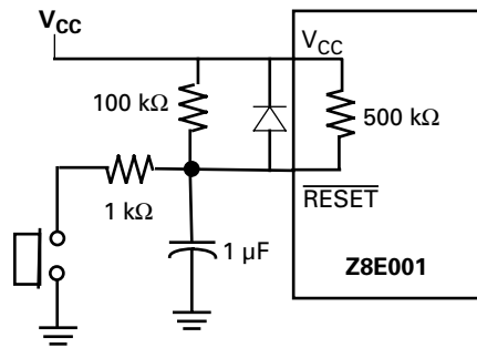
Figure 10. Example of External Power-On Reset (POR) Circuit
