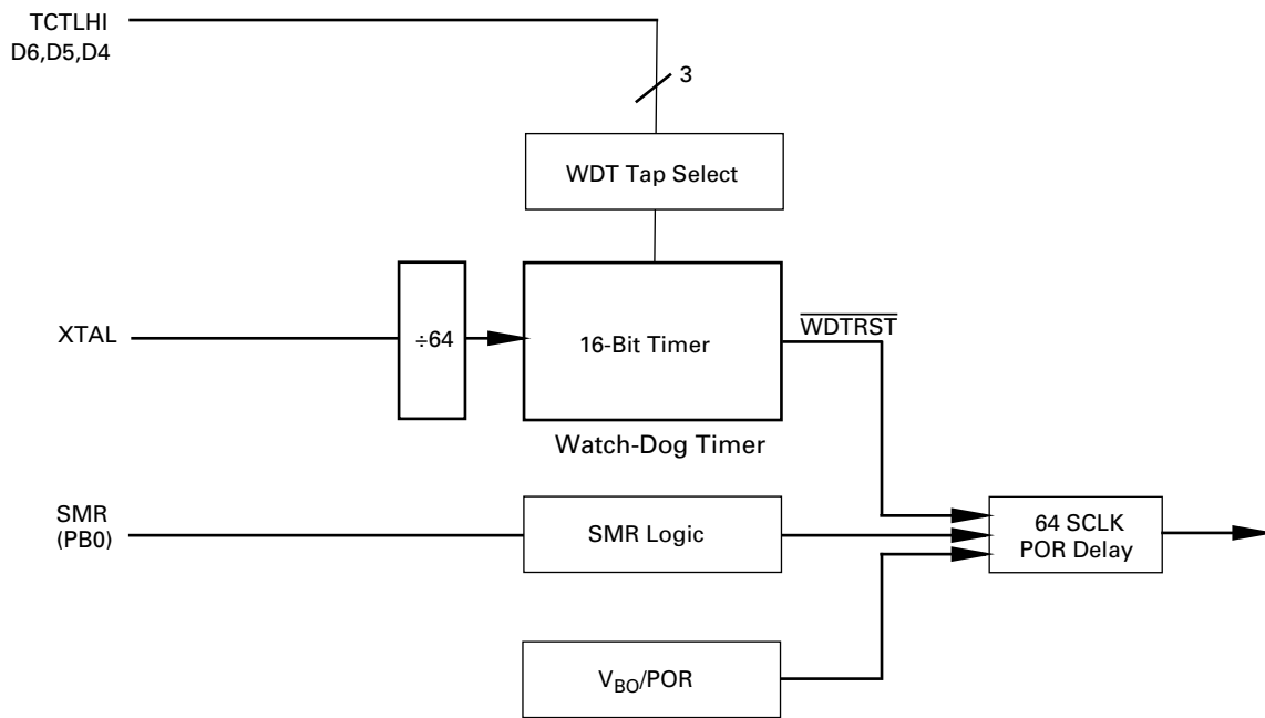
Figure 11. Reset Circuitry with POR, WDT, V BO , and SMR
