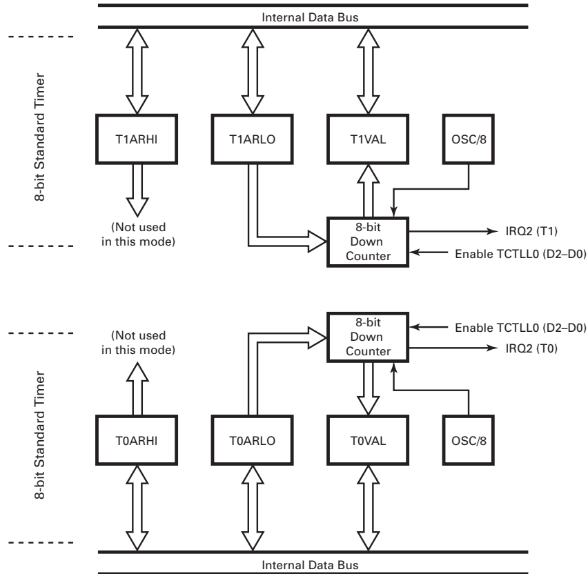
Figure 21. 8-Bit Standard Timers
