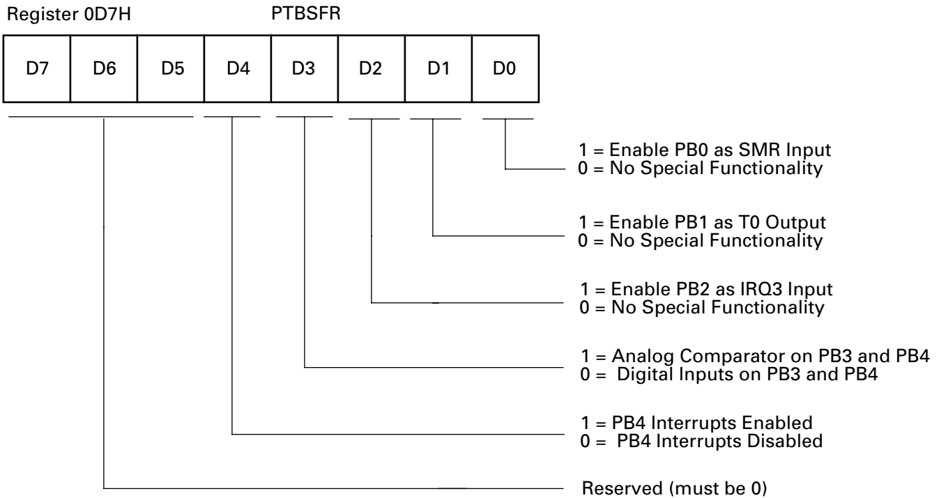
Figure 33. Port B Special Function Register
