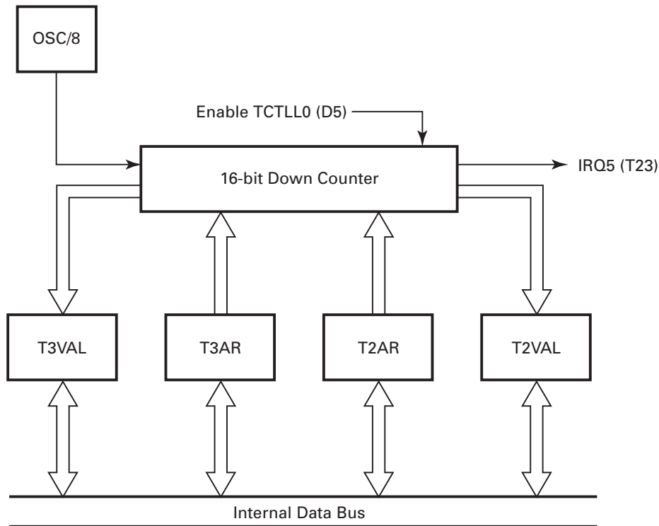
Figure 20. 16-Bit Standard Timer
