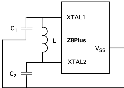
Figure 18. LC Clock
