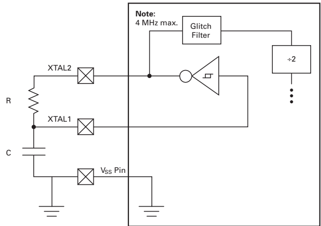
Figure 14. Z8Plus in RC Oscillator Mode
