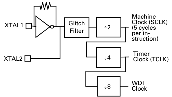
Figure 13. Clock Circuit
