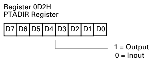
Figure 28. Port A Directional Control Register
