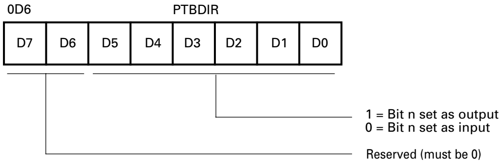
Figure 25. Port B Directional Control Register
