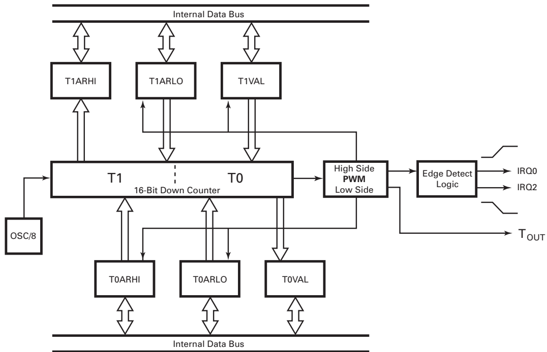
Figure 22. 16-Bit Standard PWM Timer
