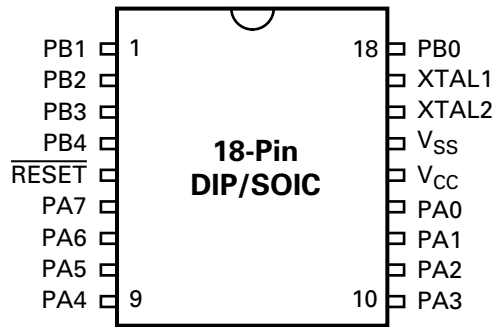
Figure 3. 18-Pin DIP/SOIC Pin Identification
