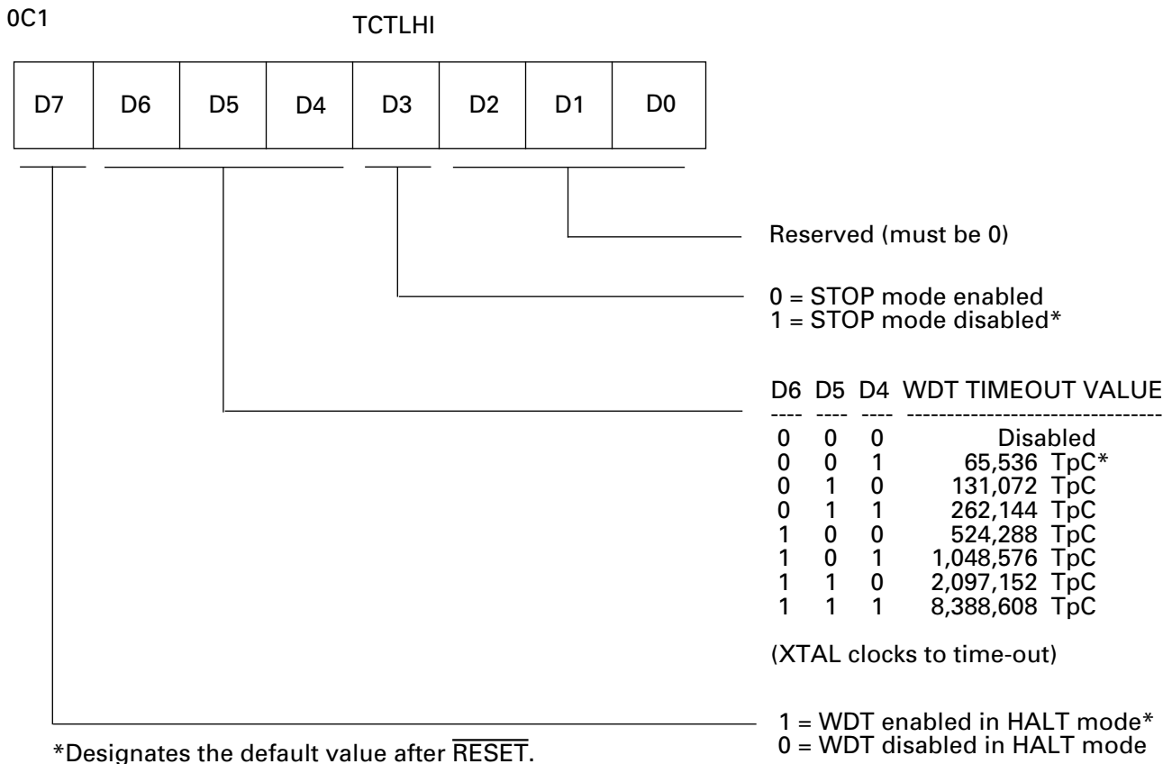
Figure 12. TCTLHI Register for Control of WDT
