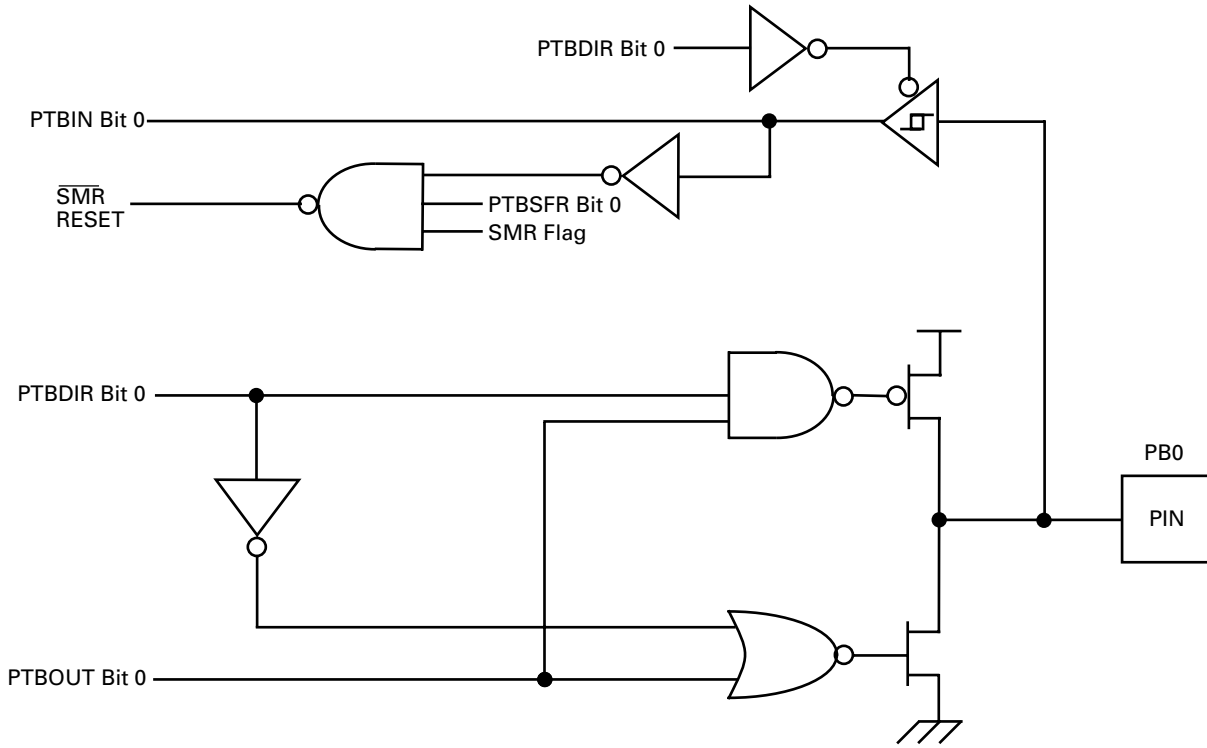
Figure 34. Port B Pin 0 Diagram
