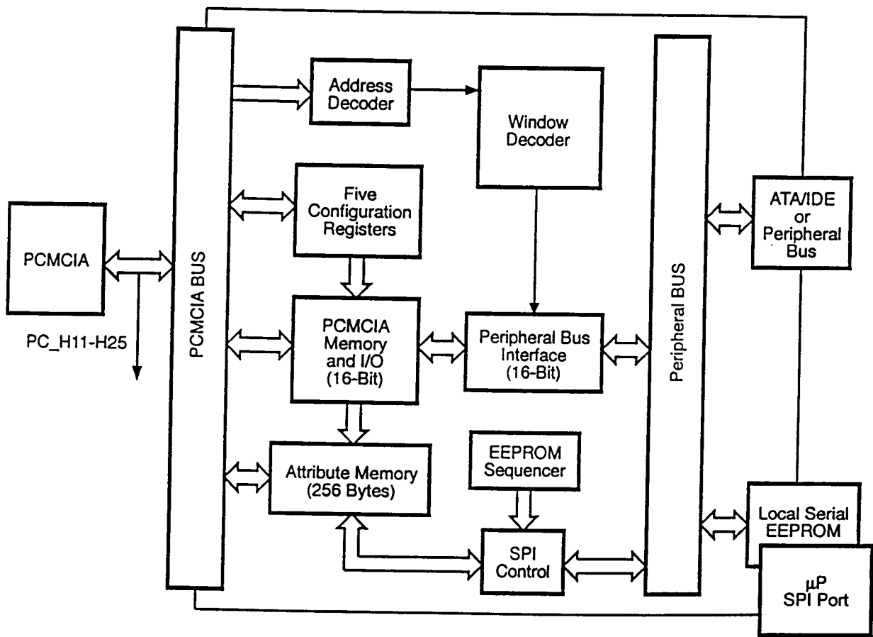
Figure 1. Z16017/Z16M17 Functional Block Diagram
