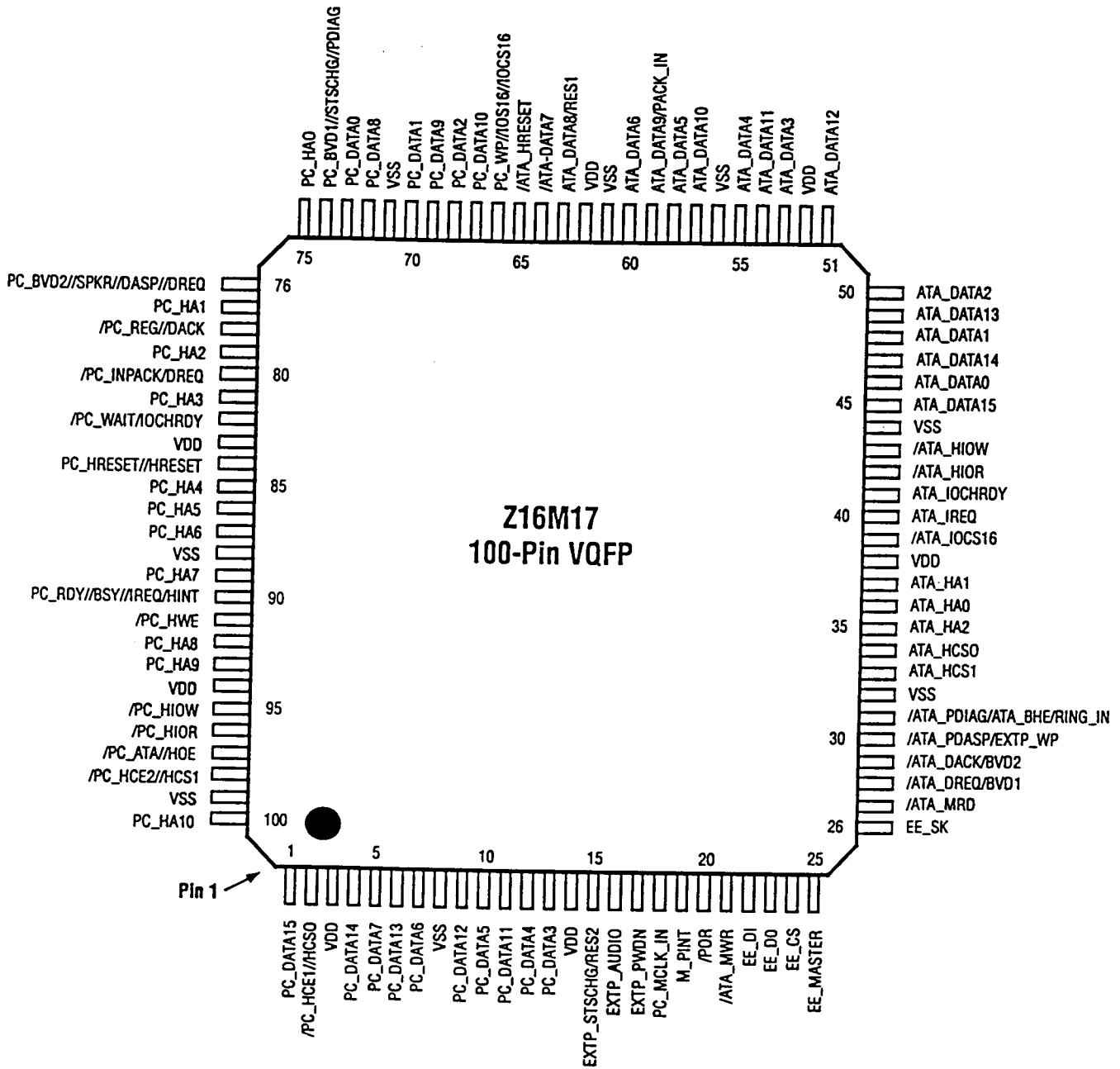
Figure 6. Z16M1720ASC1868 100-Pin VQFP Package Diagram
