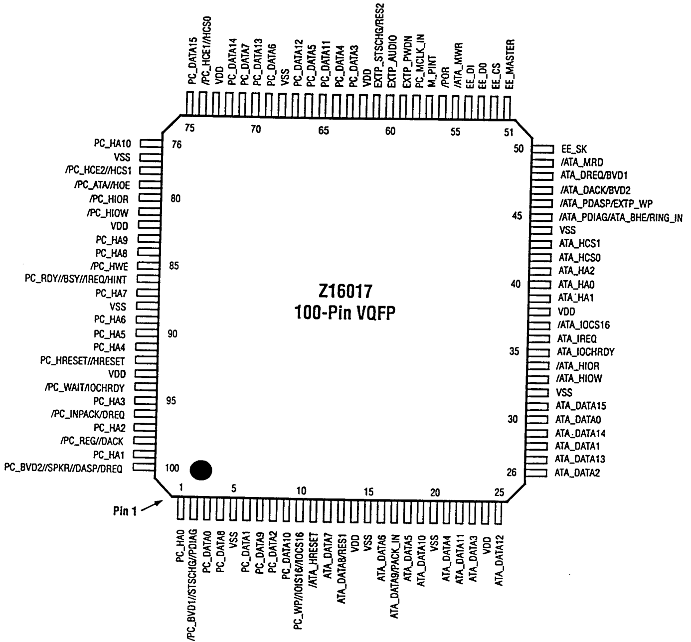
Figure 5. Z16017Z0ASC1868 100-Pin VQFP Package Diagram
