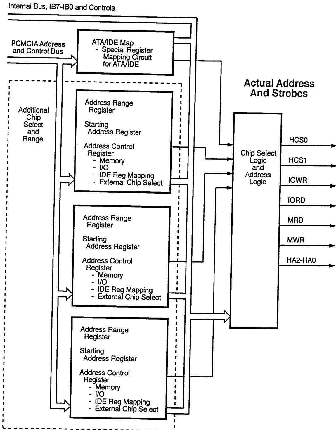
Figure 2. Connection Block Diagram PS011001-0601 - Preliminary
