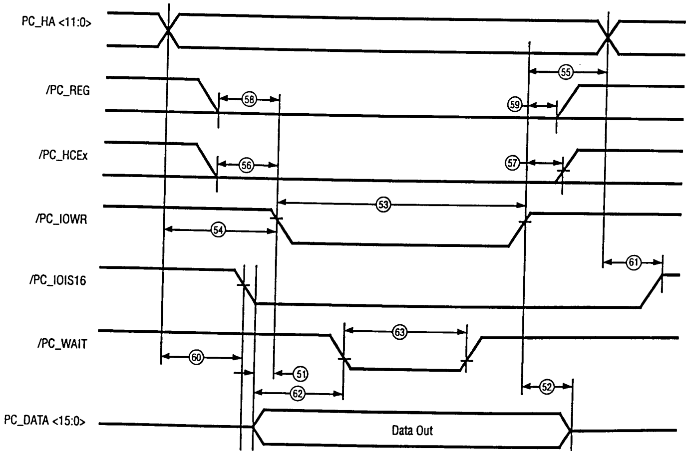
Figure 13. I/O Write Timing
