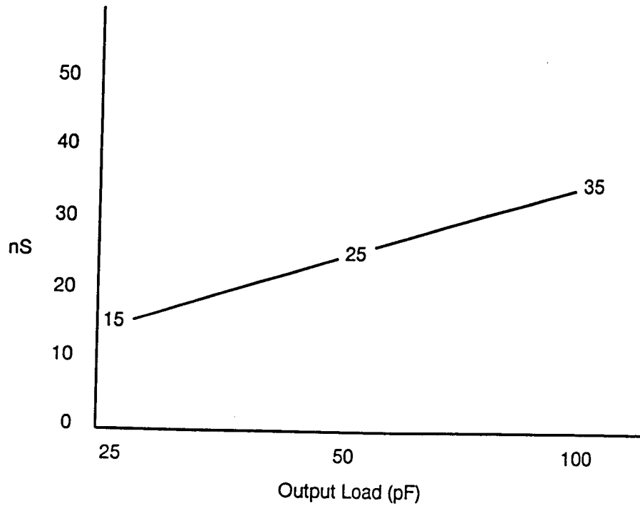
Figure 15. Z16017/Z16M17 Slew Delay Derating Curve (Typical)
