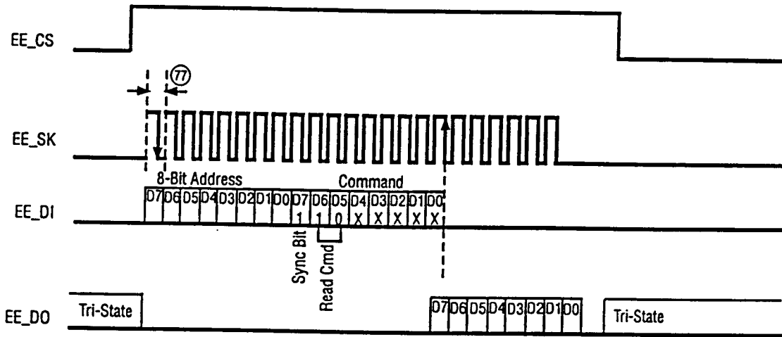
Slave Read Command
