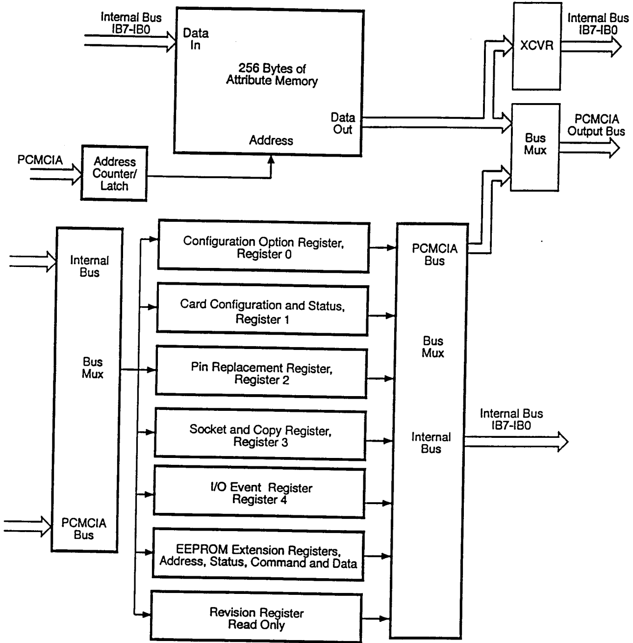
Figure 4. Attribute and Configuration Memory Diagram
