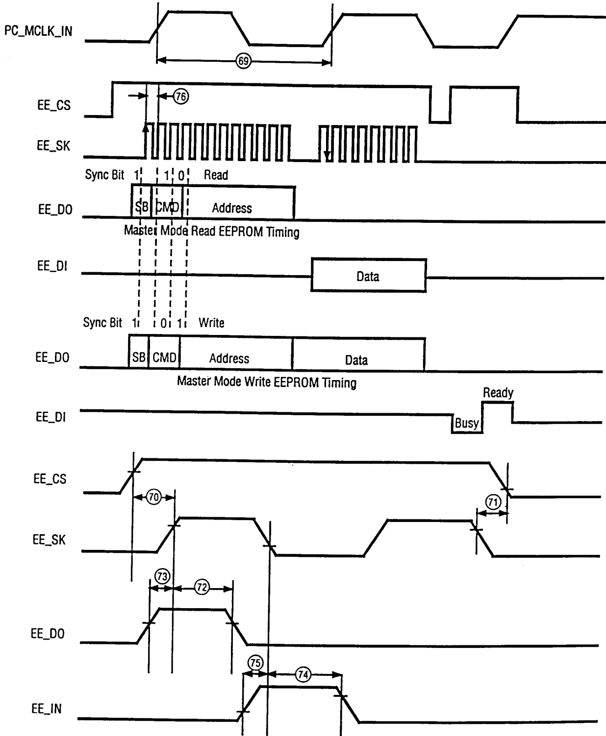
Figure 16. Master Mode Read EPROM Timing
