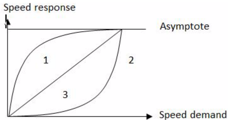
Figure 8. Non-linear Speed Response to a Linear Speed Demand
