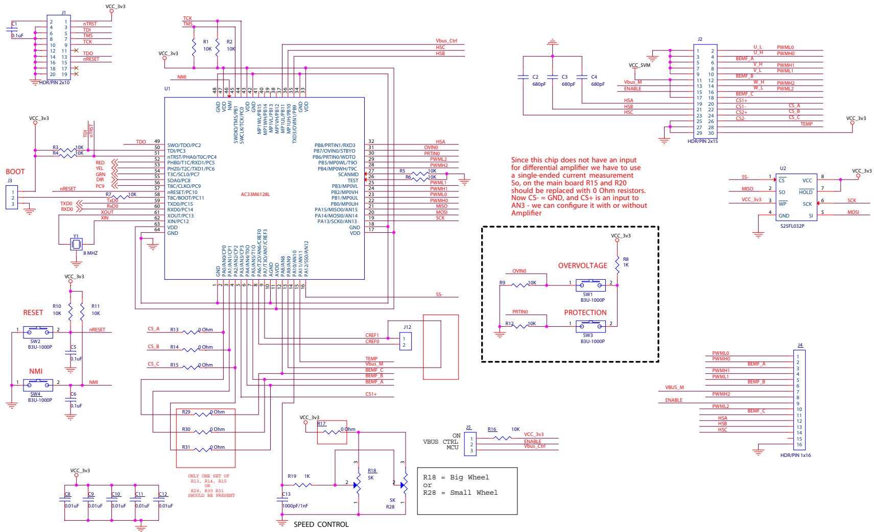
Figure 12. Z32F128 MultiMotor MCU Module, #1 of 2
