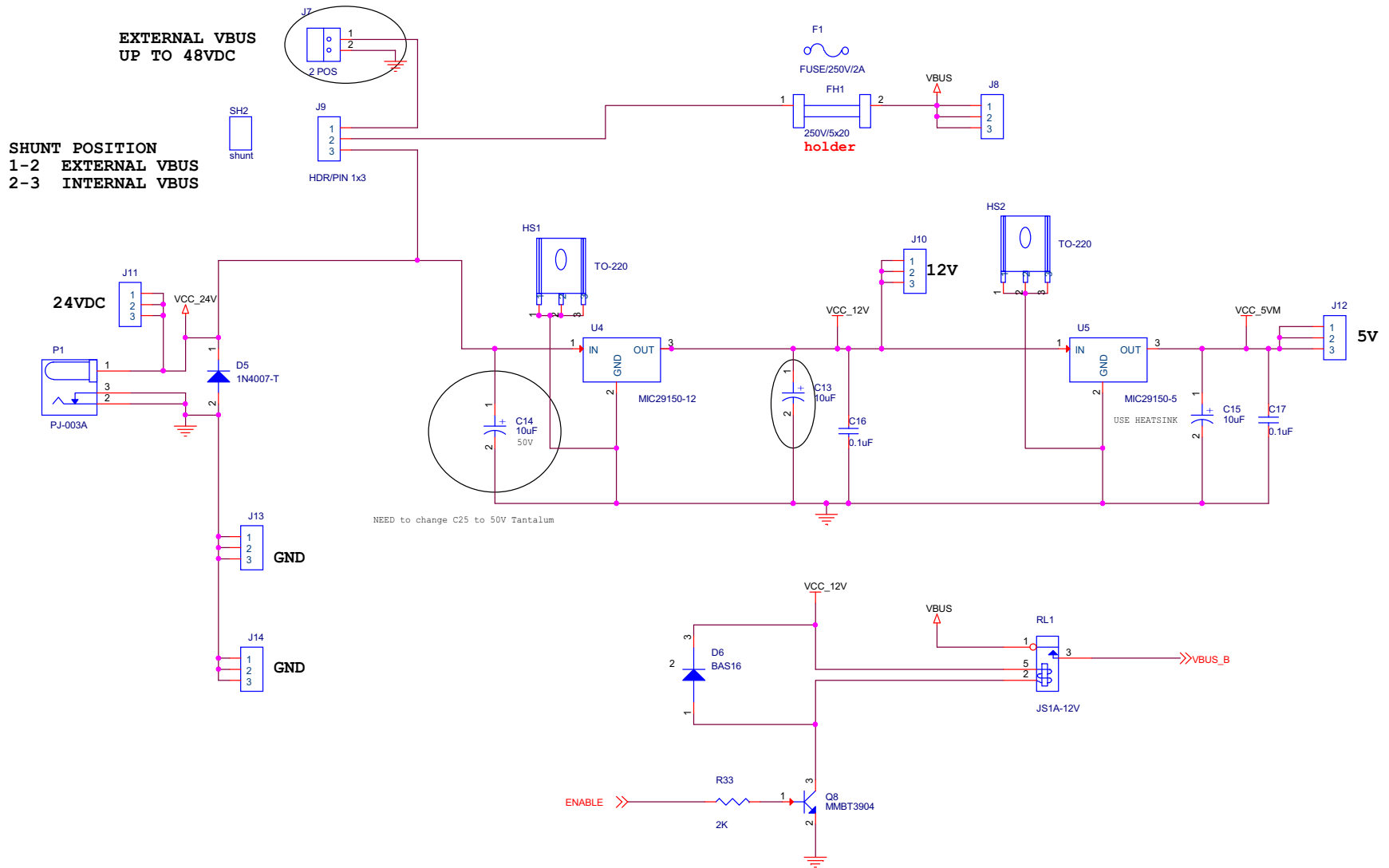
Figure 15. MultiMotor Development Board, #2 of 2
