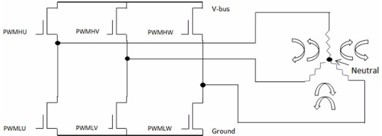
Figure 5. Inverter Bridge and AB-AC-BC-BA-CA-CB Phase Energizing Sequence with respect to Neutral
