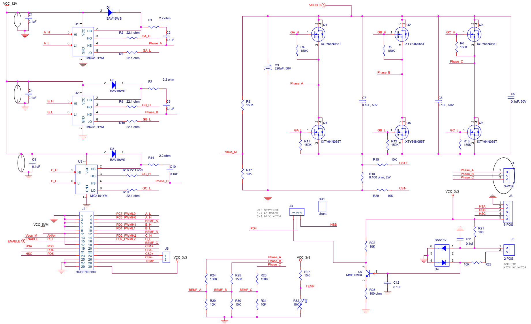
Figure 14. MultiMotor Development Board, #1 of 2
