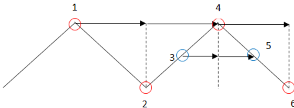
Figure 7. [Zero Crossing and Switching Timing
