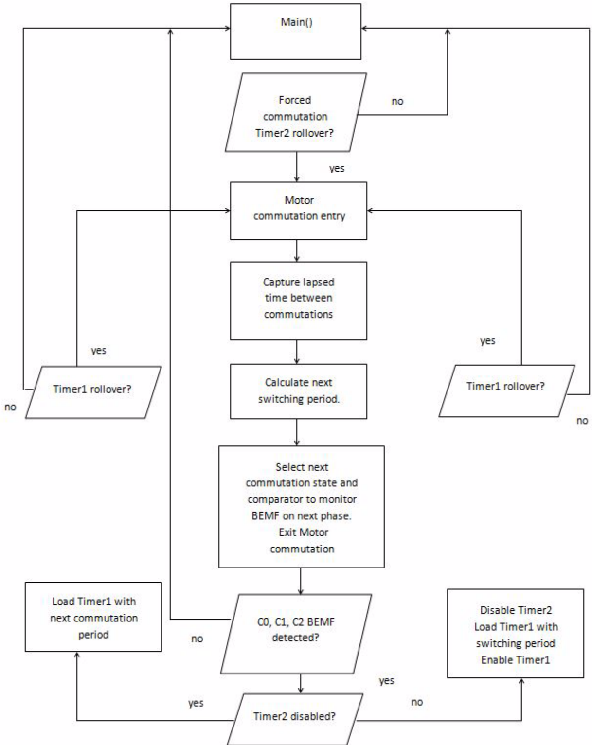
Figure 16. Forced Commutation and Commutation Based on BEMF Detection Flowchart
