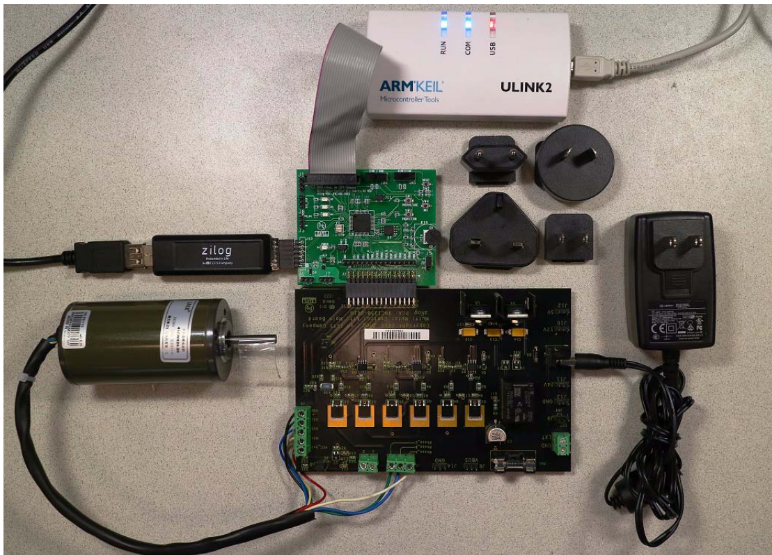
Figure 10. The MultiMotor Development Kit
