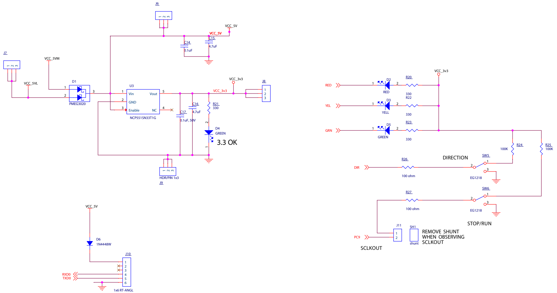
Figure 13. Z32F128 MultiMotor MCU Module, #2 of 2
