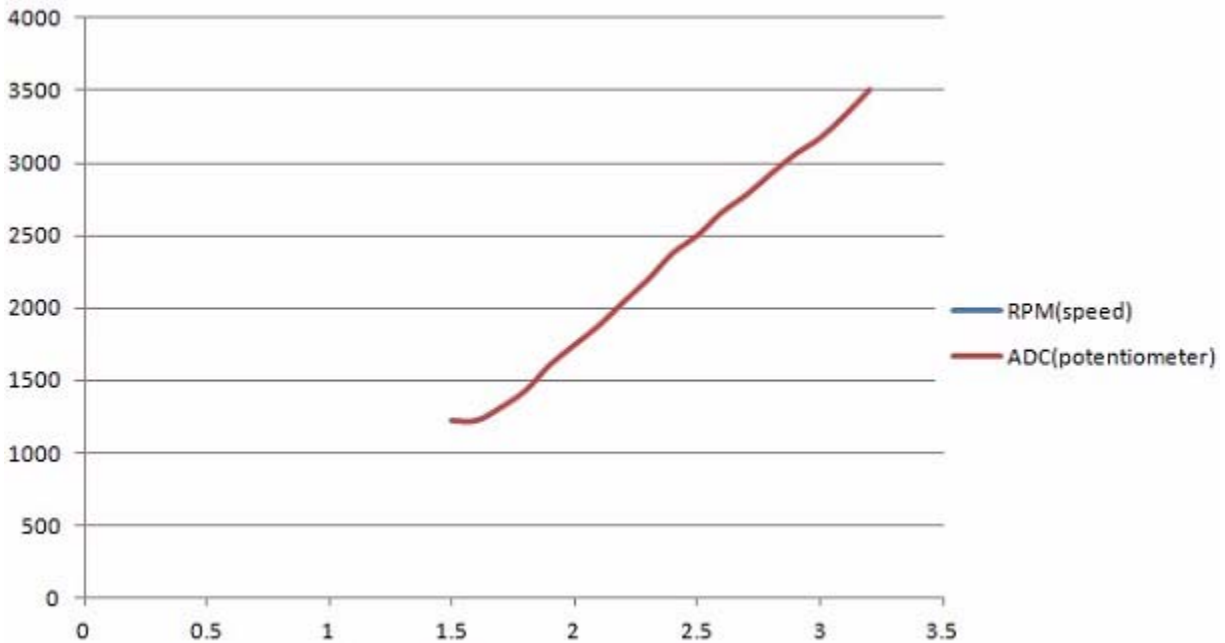
Figure 9. Speed Linearization
