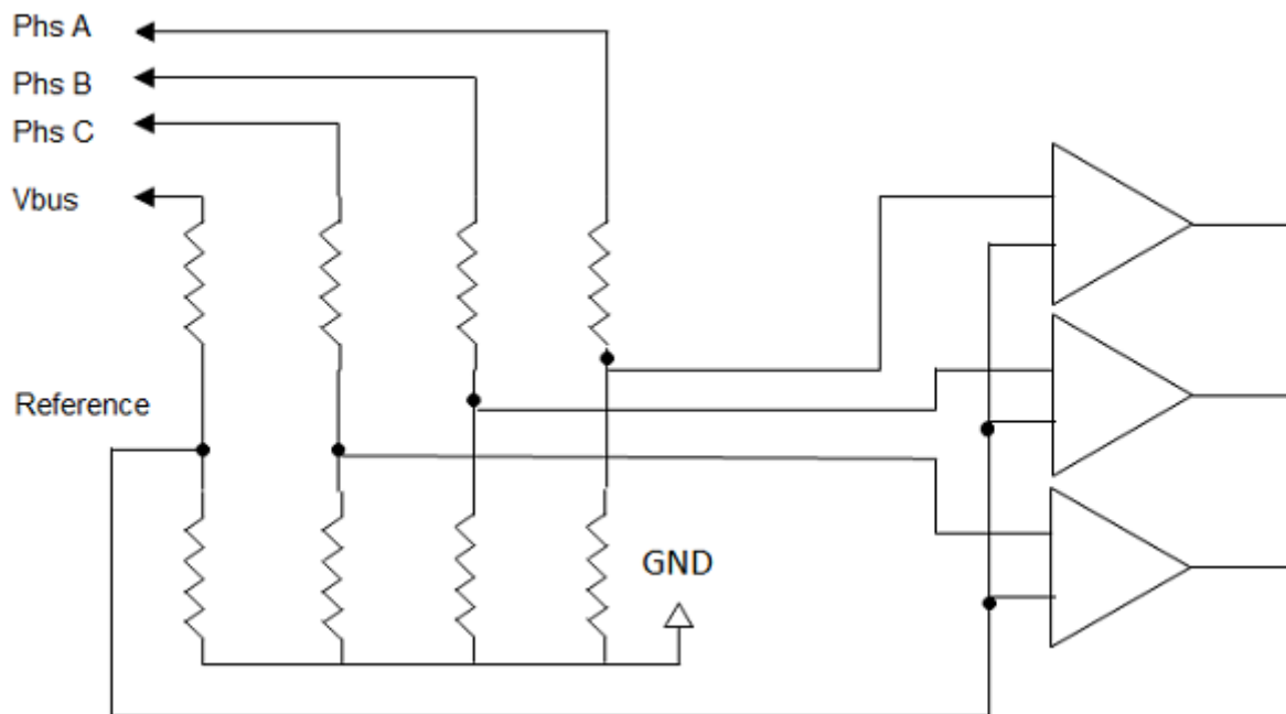
Figure 2. Three Comparators and the Resistor Network
