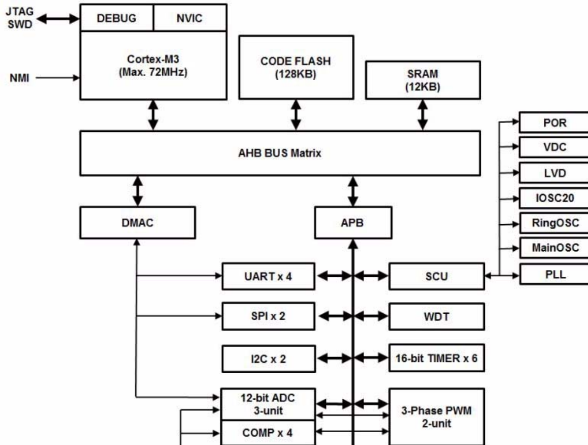
Figure 1. Z32F128 MCU Block Diagram
