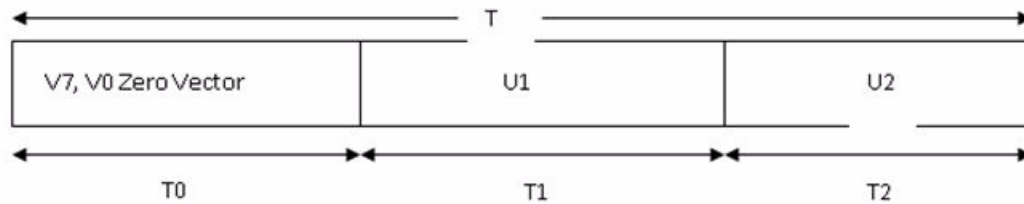
Figure 6. The Switching Times for Base Vectors V1, V2, and Zero Vectors
