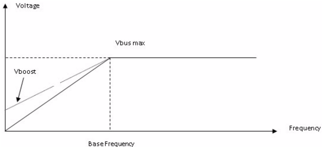
Figure 9. Voltage Per Hertz Control
