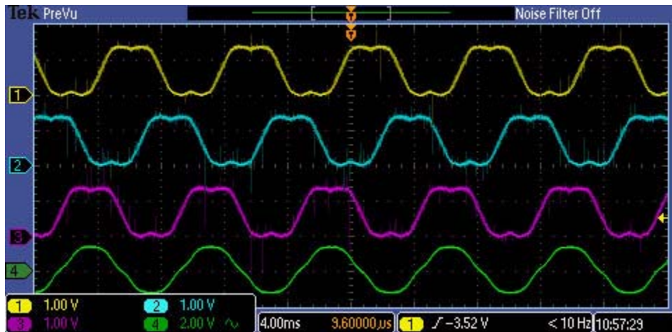
Figure 19. Three Phase Voltages and One Current Wave Form (Green)
