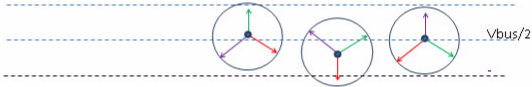
Figure 3. Space Vector Modulated Phase Voltages not Confined to a Neutral Point
