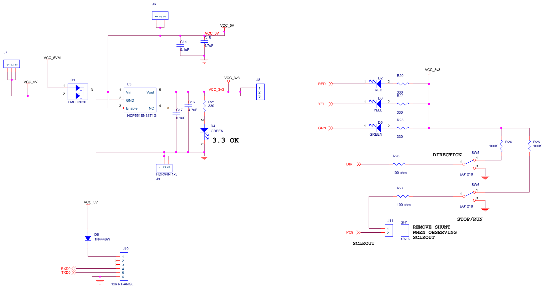
Figure 21. Z32F128 MCU Module, #2 of 2
