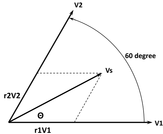
Figure 5. The Location of Reference Vector V_S Between Base Vectors V_1 and V_2
