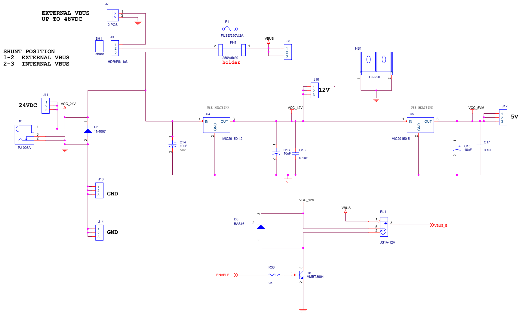
Figure 23. MultiMotor Development Board, #2 of 2
