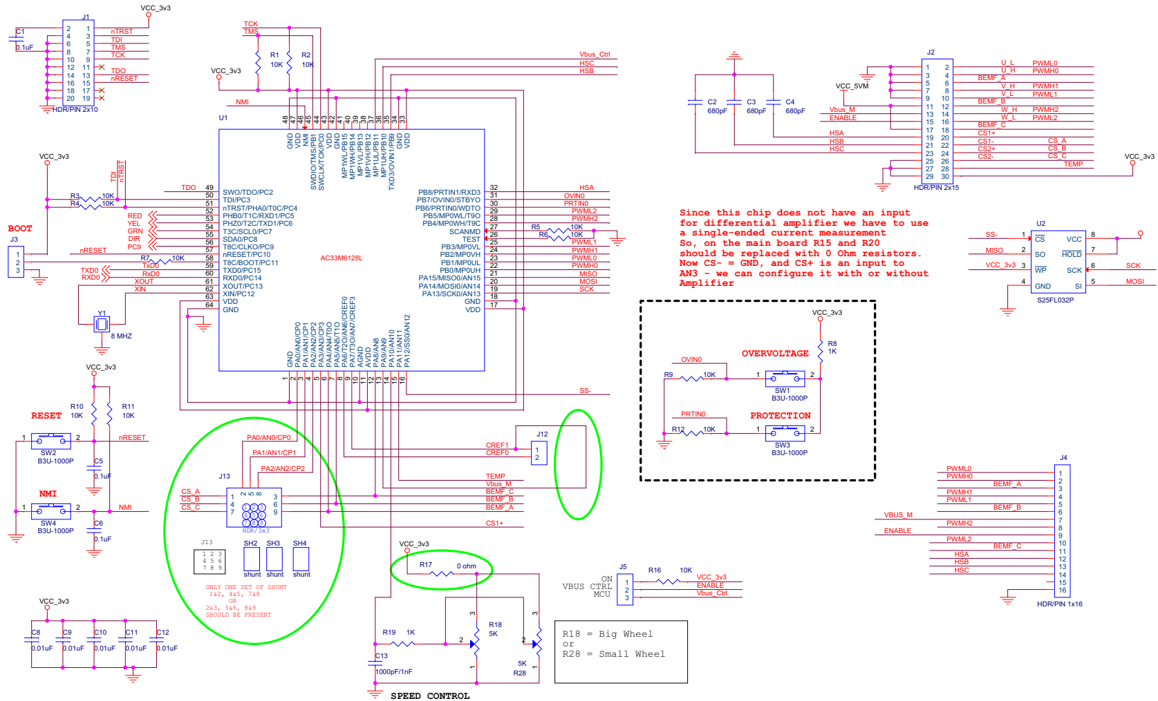
Figure 20. Z32F128 MCU Module, #1 of 2
