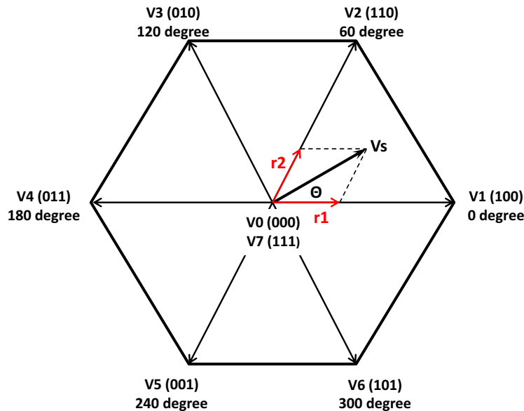
Figure 4. The Rotating Reference Vector V_{REF} Within The Hexagon
