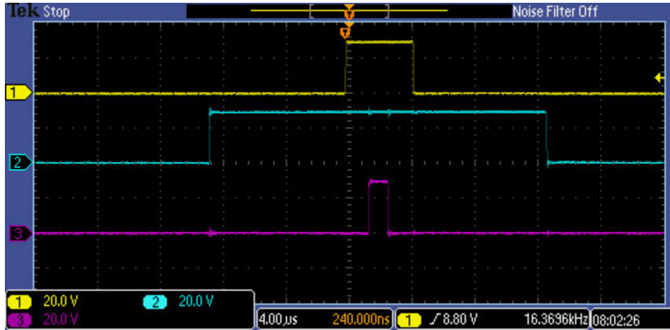
Figure 16. Alternate Switching Pattern at Time 1
