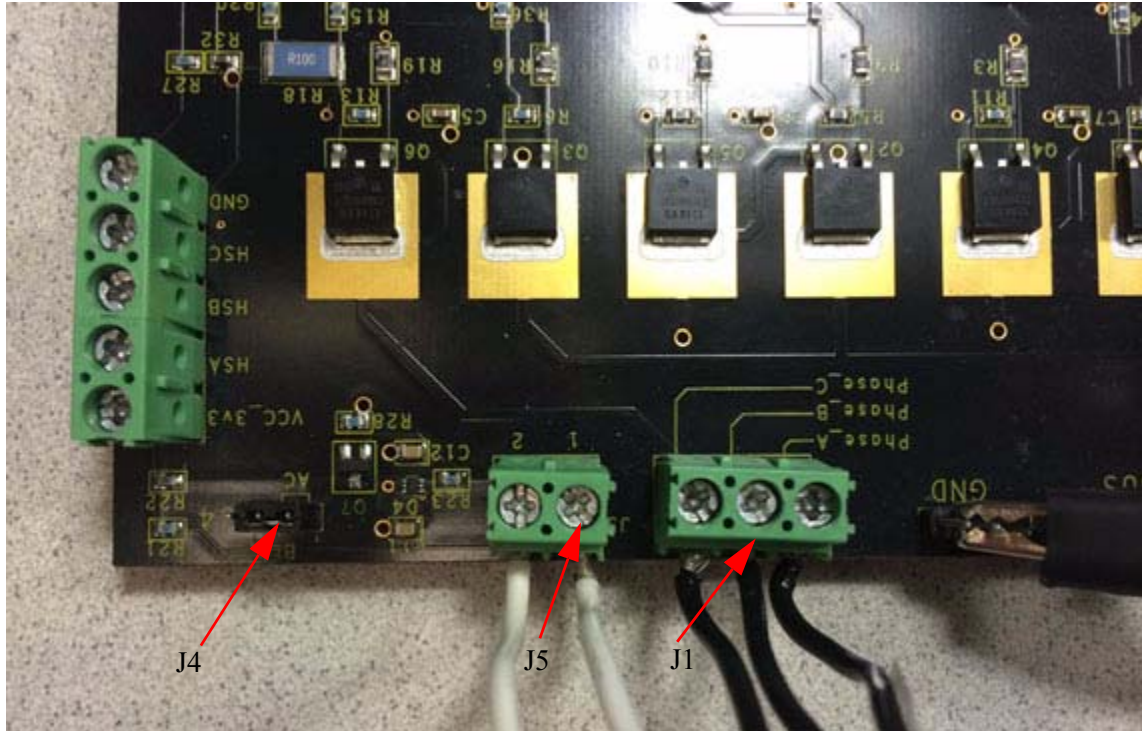
Figure 12. Motor Phase Wire Connections
