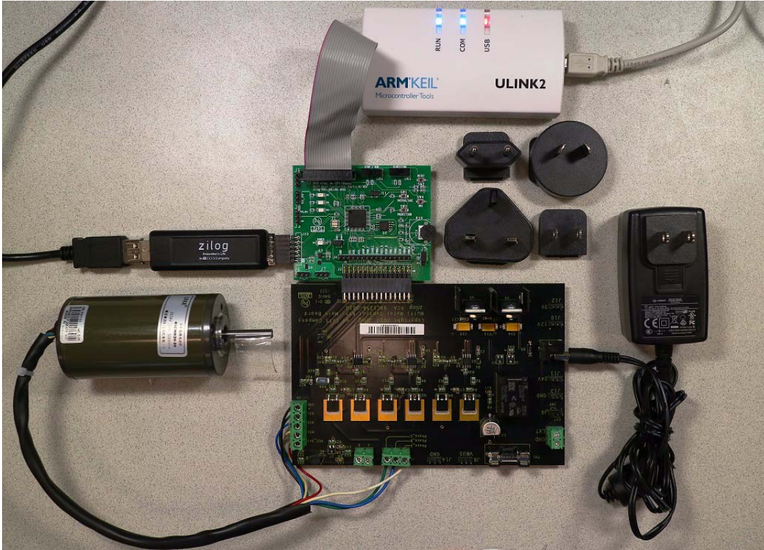
Figure 10. MultiMotor Demo Kit and Linux BLDC Motor
