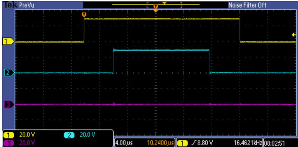
Figure 18. Alternate Switching Pattern at Time 3
