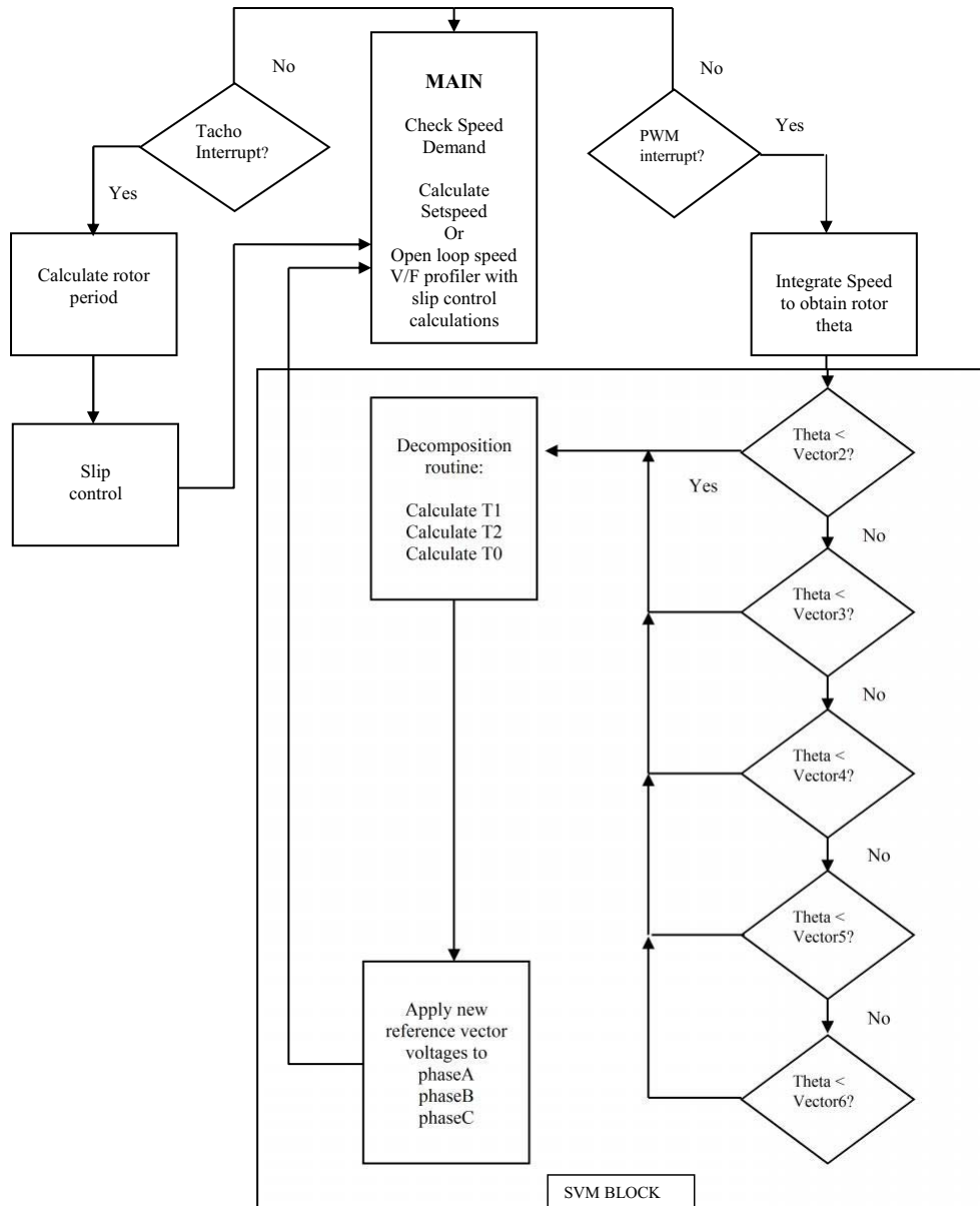
Figure 24. Space Vector Modulation Flow Chart
