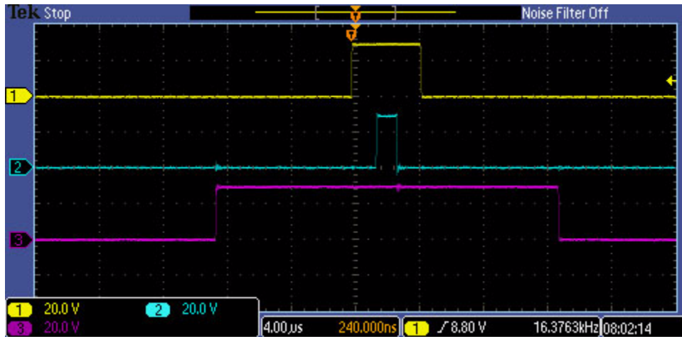
Figure 17. Alternate Switching Pattern at Time 2
